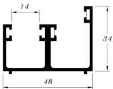
AL-69 0.768 kg/m
