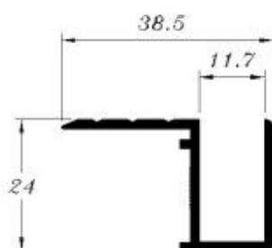
AL-5 0.550 kg/m
